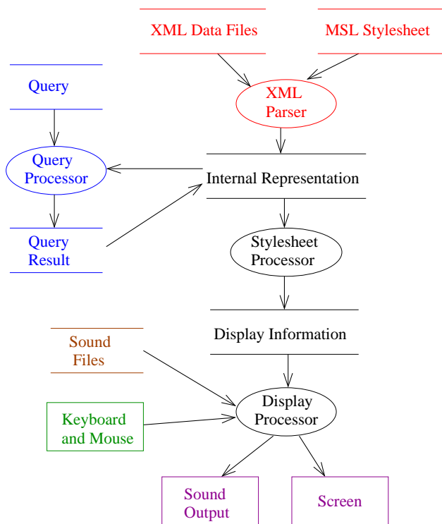
Figure 1: The MATE workbench architecture
